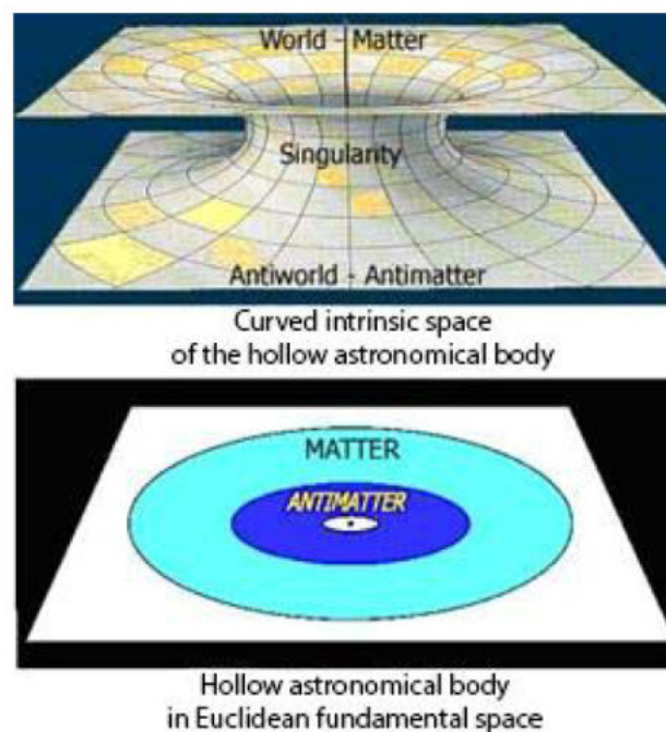
Fig. Curved intrinsic space of the hollow astronomical body and this body in Euclidean fundamental space of CFREU.
